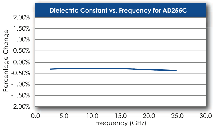
Figure 1 Demonstrates the Stability of Dielectric Constant across Frequency. This information was correlated from data generated by using a free space and circular resonator cavity. This characteristic demonstrates the inherent robustness of Arlon Laminates across Frequency, thus simplifying the final design process when working across EM spectrum. The stability of the Dielectric Constant of AD255C over frequency ensures easy design transition and scalability of design.
