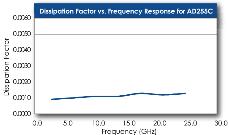
Figure 2 Demonstrates the Stability of Dissipation Factor across Frequency. This characteristic demonstrates the inherent robustness of Arlon Laminates across Frequency, providing a stable platform for high frequency applications where signal integrity is critical to the overall performance of the application.
